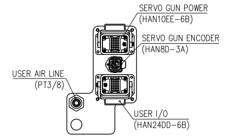
VIEW "D" (SCALE : 4/1)
