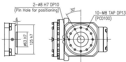
VIEW "A" (SCALE : 4/1)
