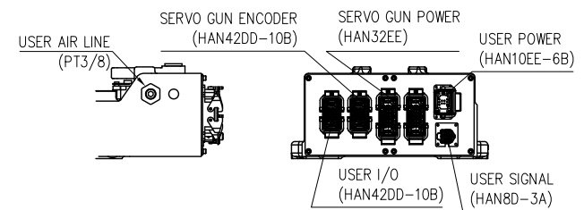
VIEW "C" <For Hi5a Controller> (SCALE : 2/1)
