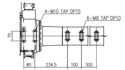
VIEW "E" (SCALE : 2/1)
