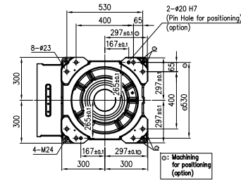
VIEW "B" (SCALE : 1/1)
