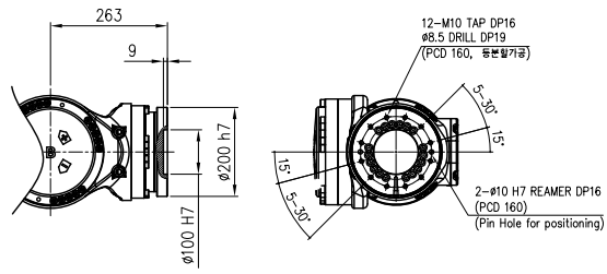
VIEW "A" (SCALE : 2/1)
