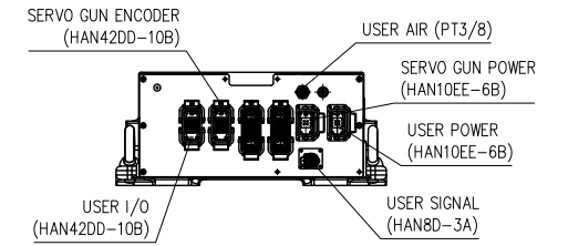
VIEW "C" (SCALE : 2/1)
