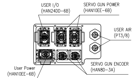
VIEW "D" (SCALE : 2/1)
